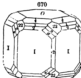
St. Gothard.
